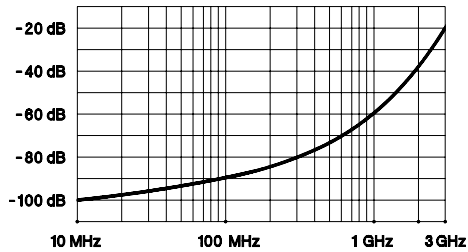
串扰 (50Ω)
